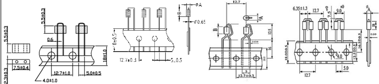
RID 2.3x5.5x7.5-0.8-L-T
