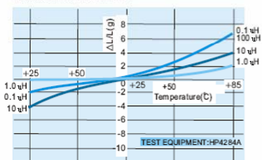
INDUCTANCE vs. TEMPERATURE CHARACTERISTICS
