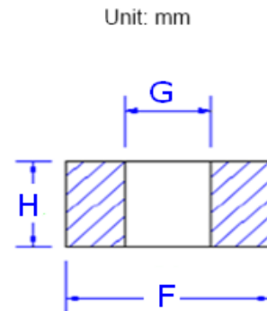
LAND PATTERN
