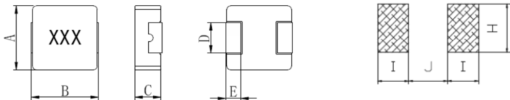
LAND PATTERN
